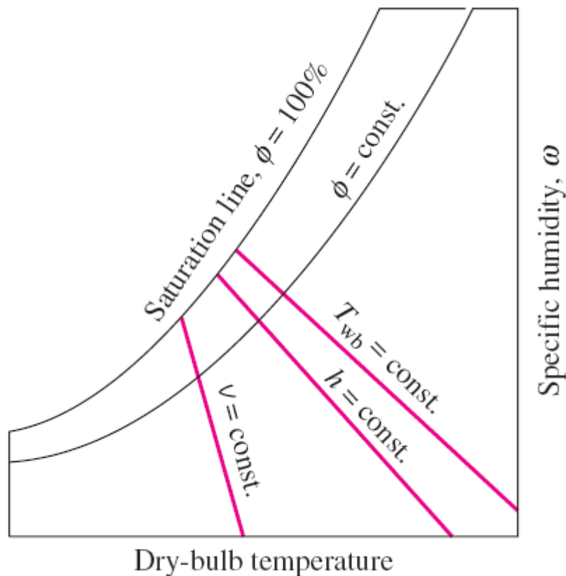
Schematic for a psychrometric chart.
