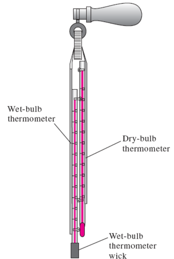
Sling psychrometer
