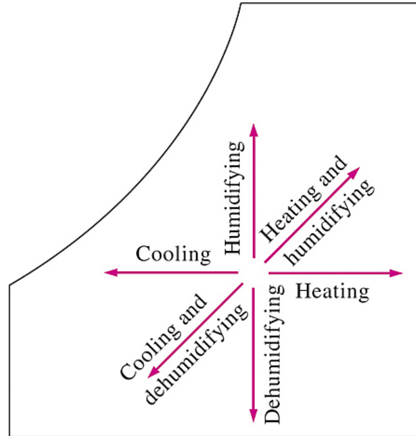
Various air-conditioning processes.
