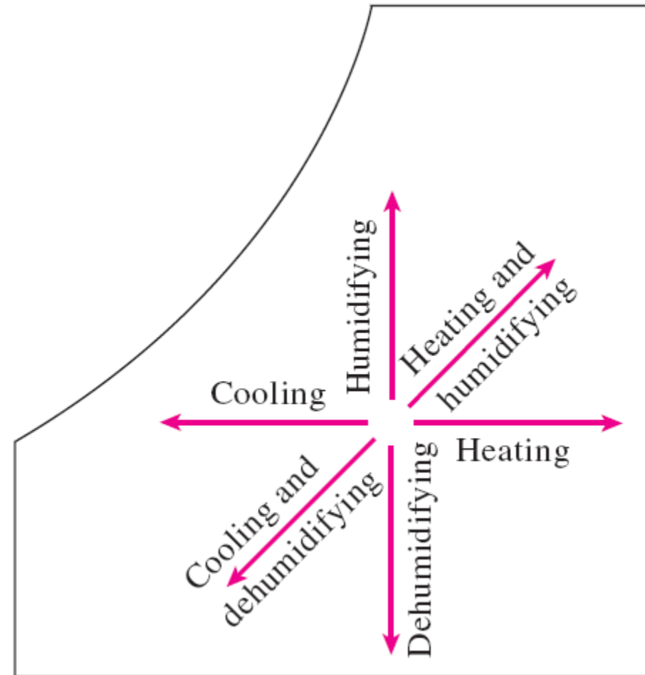
Various air-conditioning processes.
