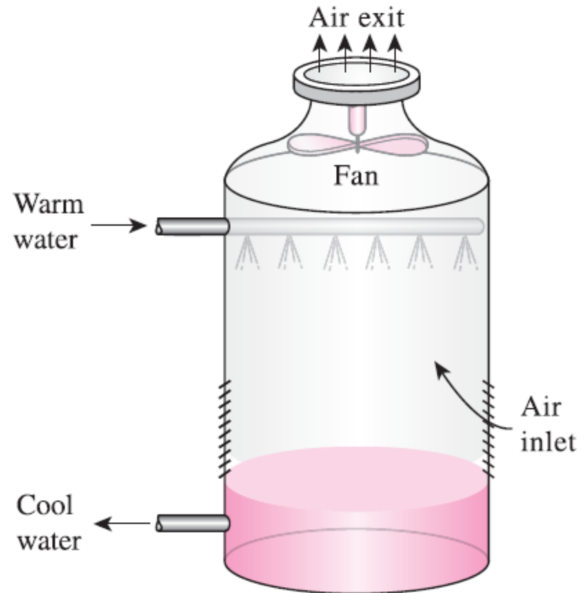
An induced-draft counterflow cooling tower.
